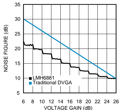
Noise Figure Over Voltage Gain Range DVGA Response Shown for Comparison
