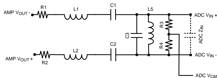
Figure 42. ADC Noise Filter Schematic
