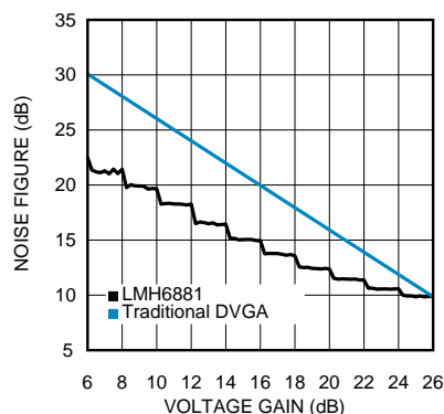
Noise Figure Over Voltage Gain Range DVGA Response Shown for Comparison
