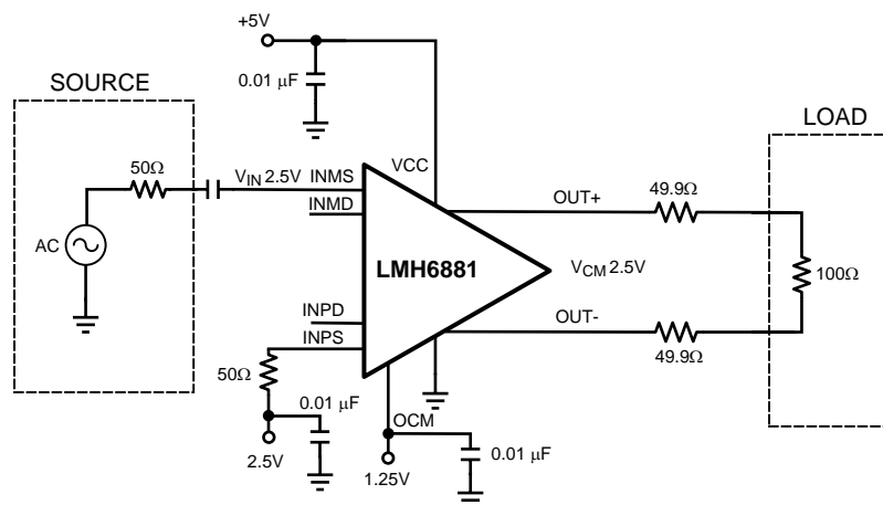
Figure 39. Typical Implementation with a Single-Ended Input Signal
