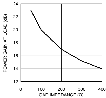
Figure 41. Power Gain as a Function of the Load
