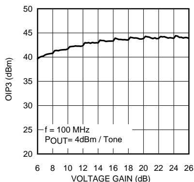
OIP3 over Voltage Gain Range
