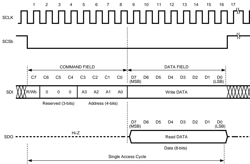
Figure 46. Serial Interface Protocol (SPI Compatible)
