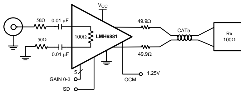
Figure 37. LMH6881 Used as Twisted Pair Cable Driver
