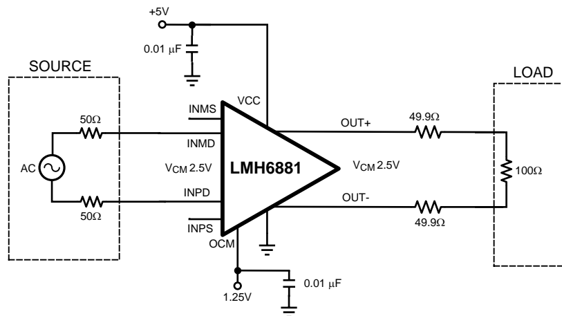
Figure 38. Typical Implementation with a Differential Input Signal
