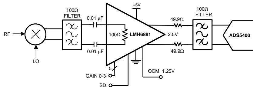
Figure 36. LMH6881 Typical Application
