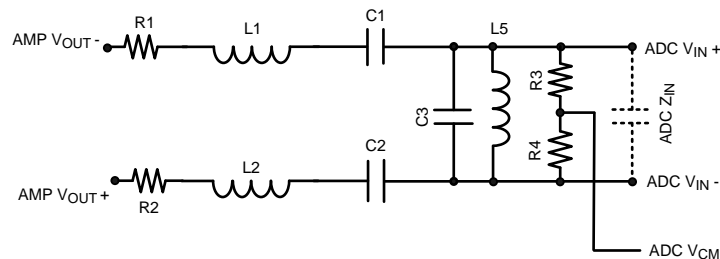
Figure 42. ADC Noise Filter Schematic
