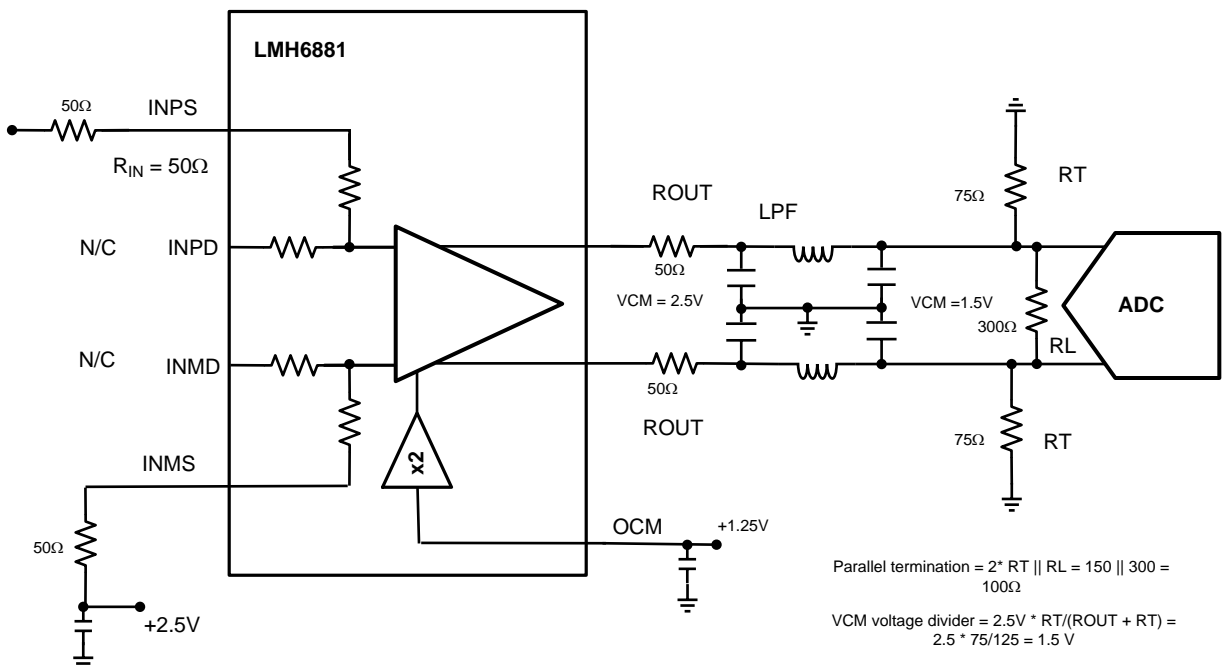
Figure 43. DC-Coupled ADC Driver Example 1, High Input Impedance ADC
