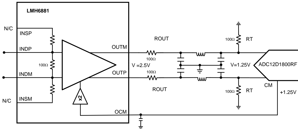
Figure 44. DC-Coupled ADC Driver Example 2, Terminated Input ADC
