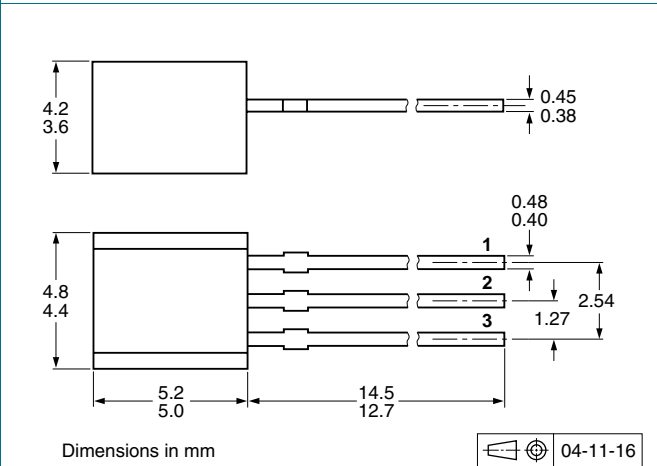
Fig 12. Package outline SOT54 (SC-43A/TO-92)
