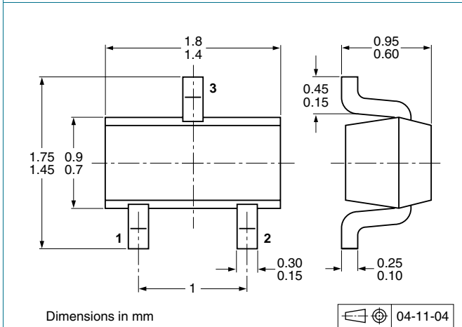
Fig 11. Package outline SOT416 (SC-75)
