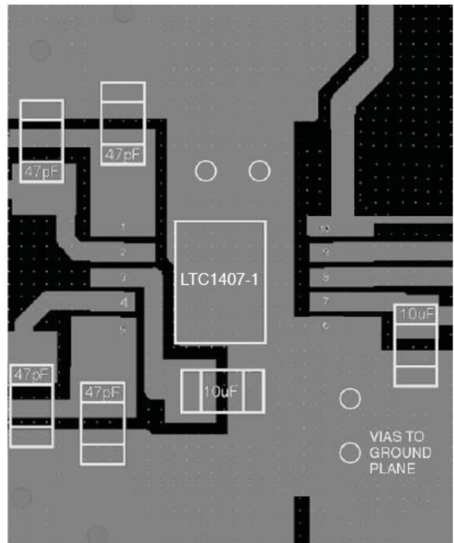
Figure 7. Recommended Layout
