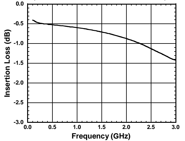
PC-P2 Insetion Loss vs. Frequency ( VCTL1=2.7V, VCTL2=0V, Pin=0dBm )
