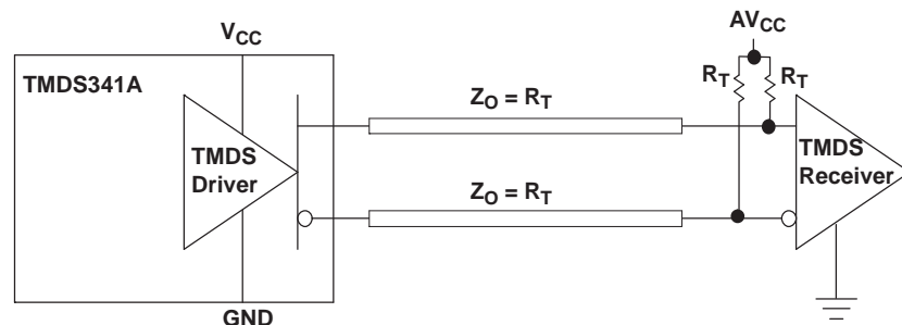
Figure 35. TMDS Driver and Termination Circuit
