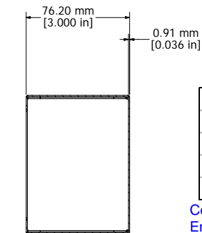
SECTION EE-EE
