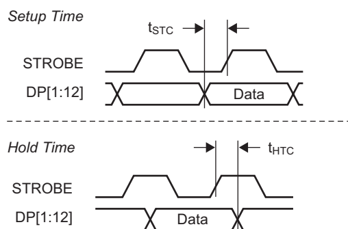
Figure 19. Serial Setup and Hold Time
