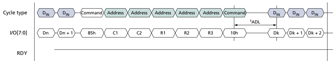
Figure 37: PROGRAM FOR INTERNAL DATA INPUT (85h) Operation
