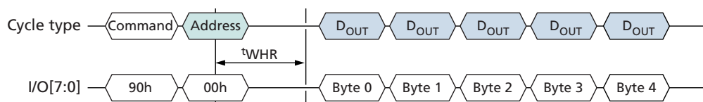
Figure 26: READ ID (90h) with 00h Address Operation
