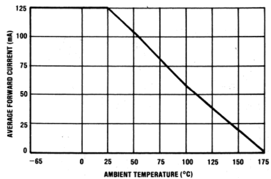
FIGURE 2 1N5181-84
