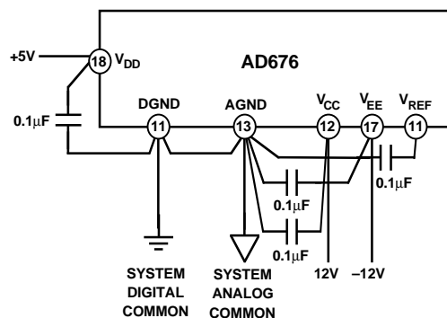
Figure 4. Grounding and Decoupling the AD676
