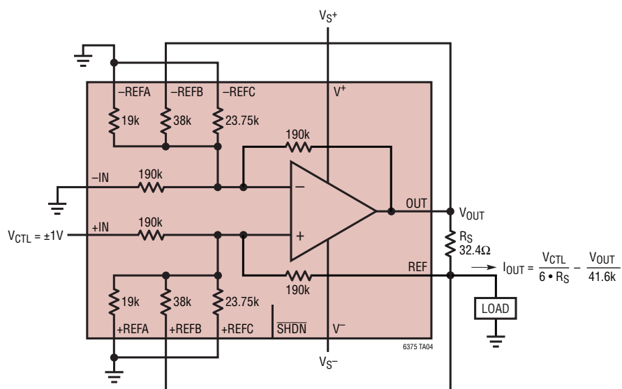
\pm 5\text{mA} Howland Current Source
