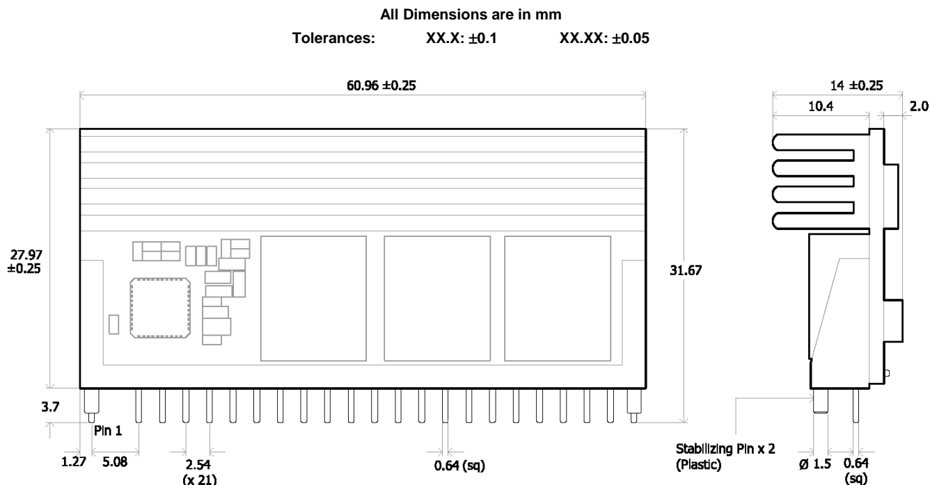
Figure 47. Mechanical Drawing
