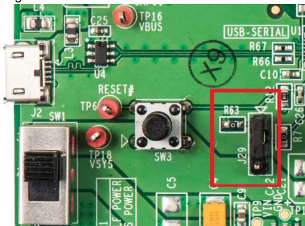
Figure 3-25. VBUS Selection
