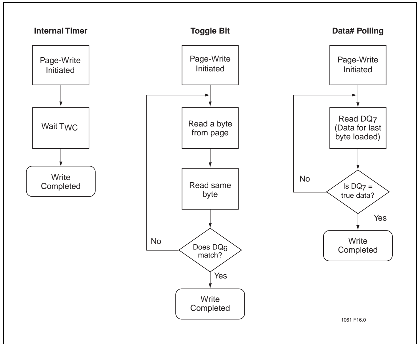
FIGURE 17: Wait Options
