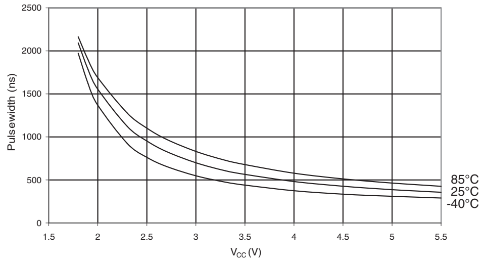
Figure 27-94. Minimum Reset Pulwidth vs. V_{CC}
