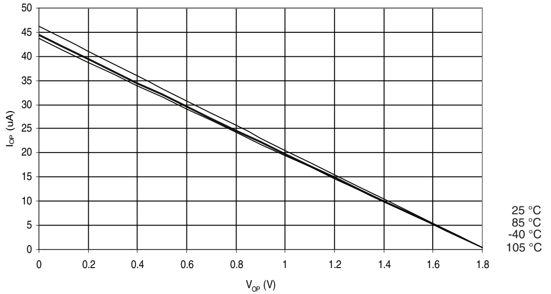
Figure 28-9. ATmega164P: I/O Pin Pull-up Resistor Current vs. Input Voltage ( V_{CC} = 1.8V )
