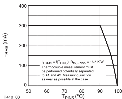
Fig. 6 - Current Reduction
