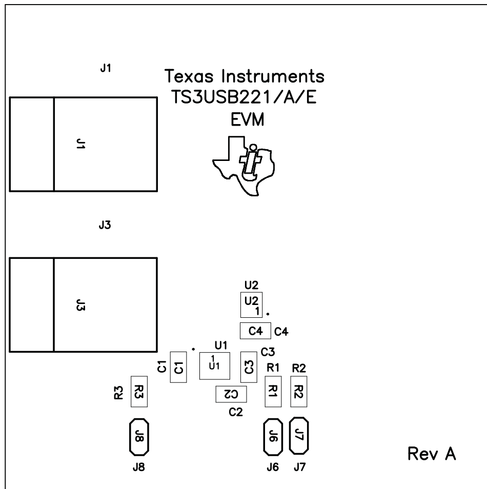
Figure 5. Top Silkscreen/Assembly
