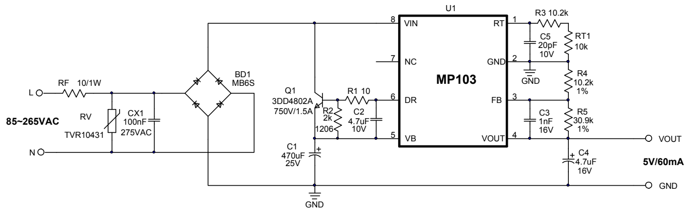
Figure 7: Typical Application
