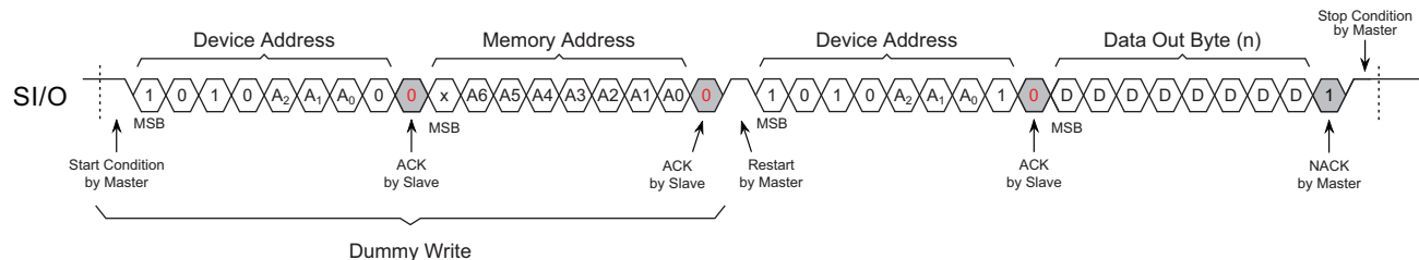
Figure 8-2. Random Read
