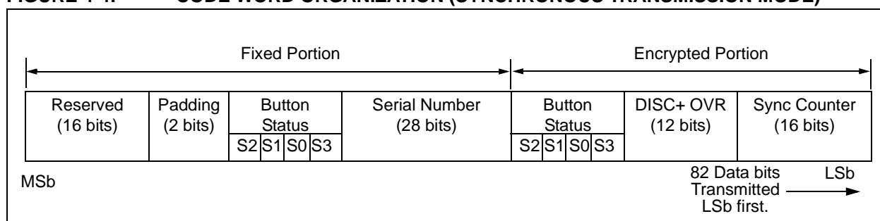
FIGURE 4-4: CODE WORD ORGANIZATION (SYNCHRONOUS TRANSMISSION MODE)
