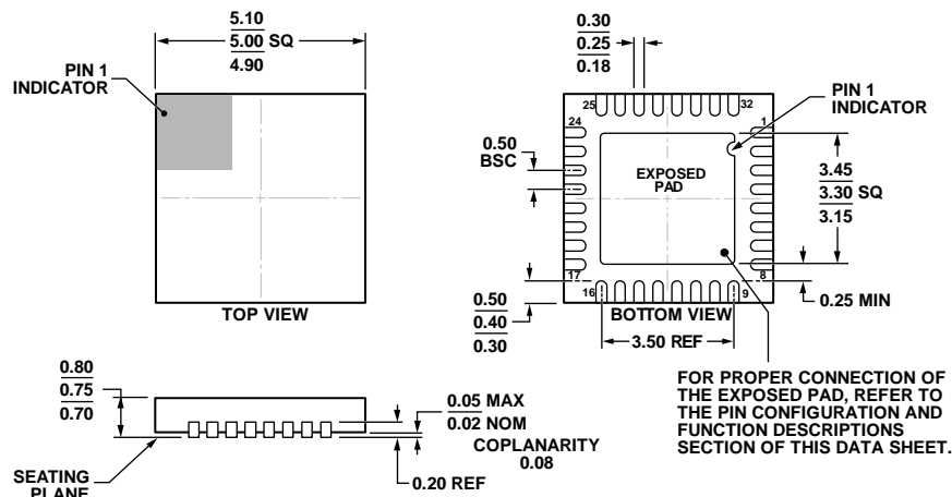
Figure 74. 32-Lead Lead Frame Chip Scale Package [LFCSP_WQ] 5 mm x 5 mm Body, Very Very Thin Quad (CP-32-13) Dimensions shown in millimeters
