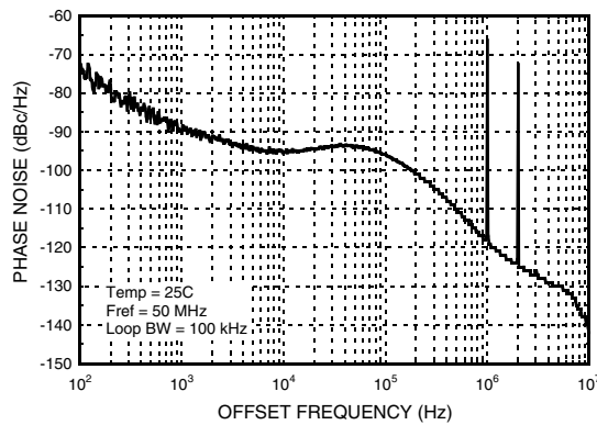
SSB Phase Noise Fractional Spurs @ 12.002 GHz
