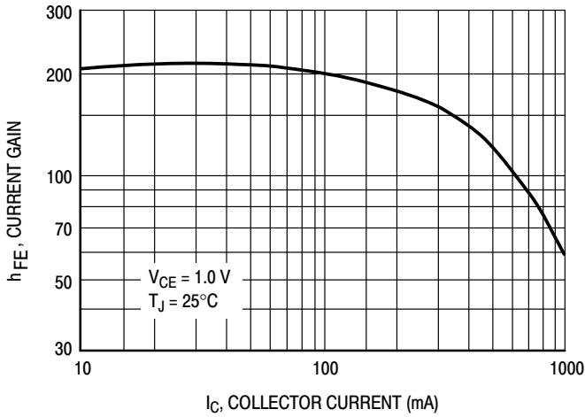
Figure 3. MPS6601/6602 DC Current Gain
