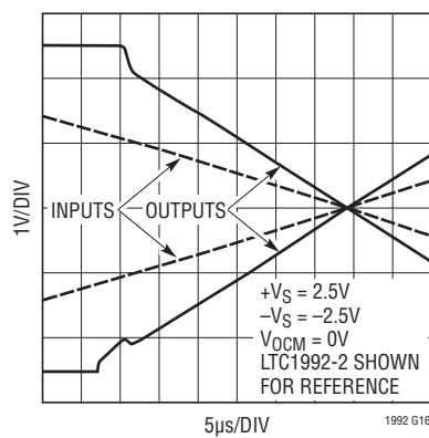
Output Overdrive Recovery (Detailed View)
