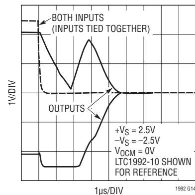
Input Common Mode Overdrive Recovery (Detailed View)
