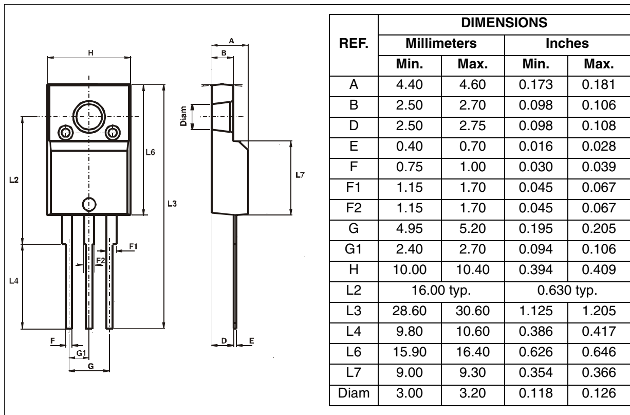
Figure 15: ISOWATT220AB Package Mechanical Data
