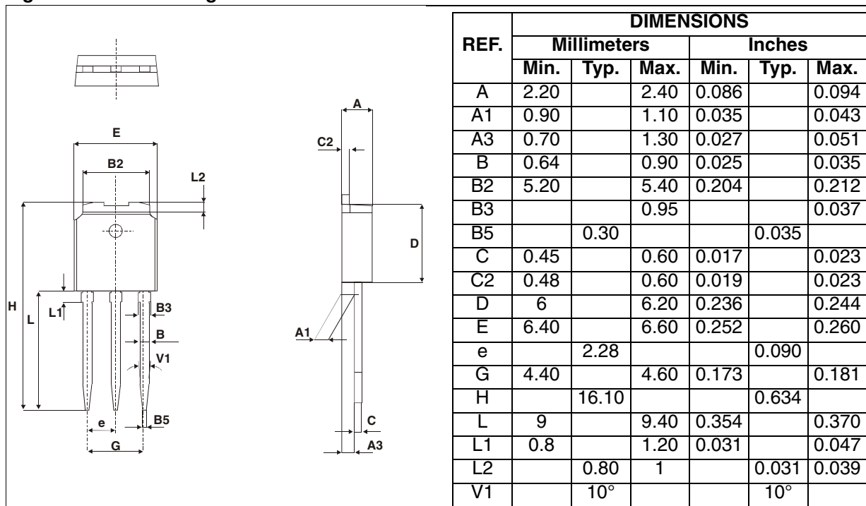
Figure 16: IPAK Package Mechanical Data
