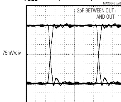
ELECTRICAL EYE DIAGRAM ( I_{MOD} = 30mA , 622.08MHz, 2 7 - 1 PRBS)
