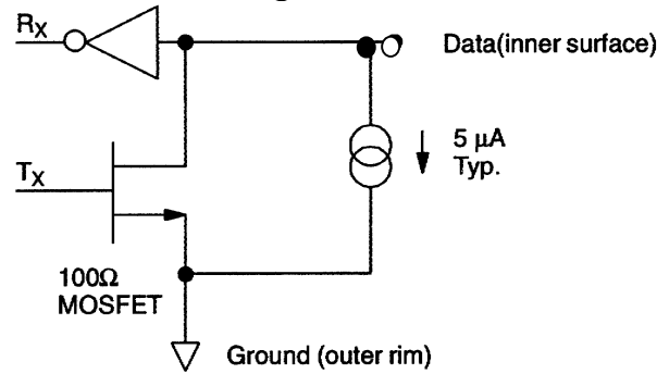
DS1990A EQUIVALENT CIRCUIT Figure 2
