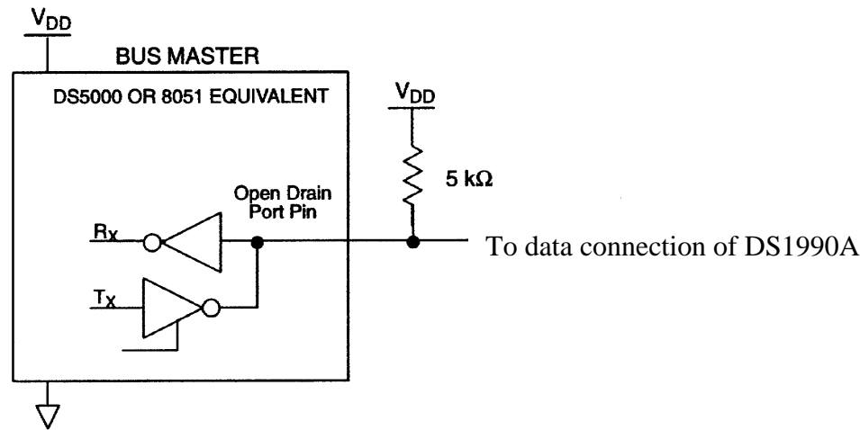
BUS MASTER CIRCUIT Figure 3
