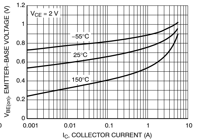
Figure 7. V_{BE(on)} Voltage
