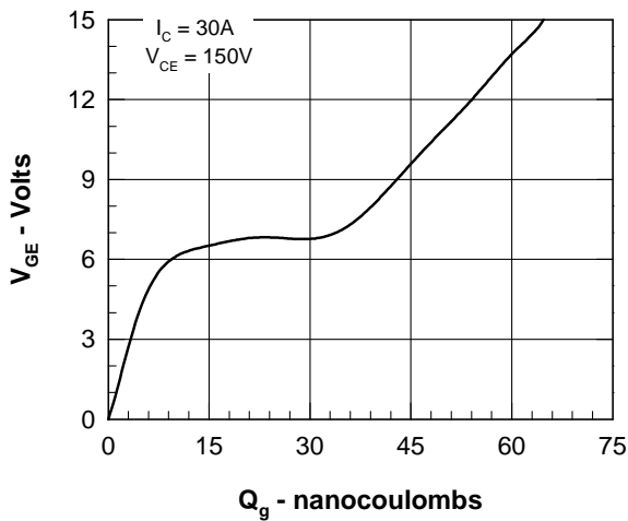
Figure 9. Gate Charge
