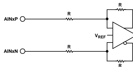
Figure 16. Analog Input Block
