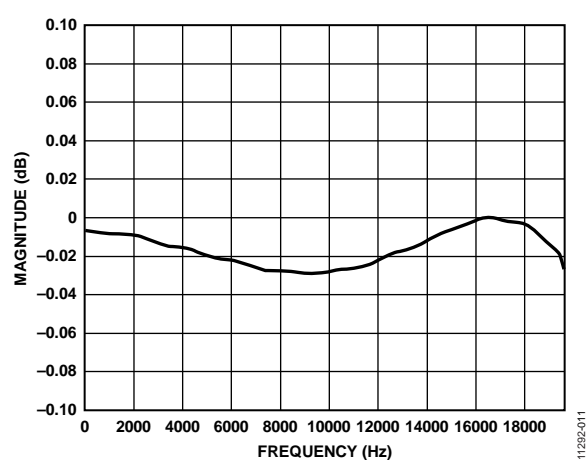
Figure 11. ADC Pass-Band Ripple at f_s = 48 kHz
