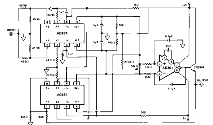
FREQUENCY DOUBLER
