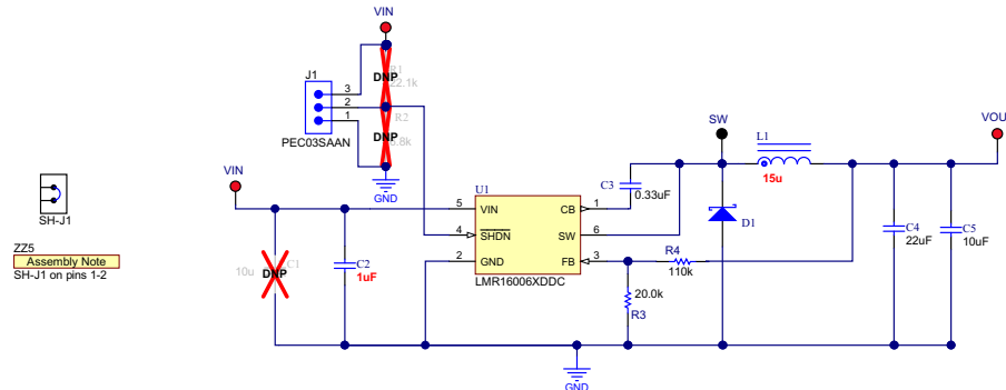
Figure 5. LMR1606XEVM Schematic
