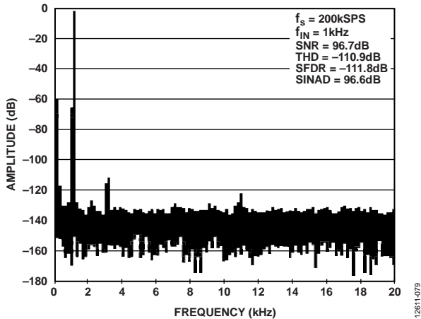
Figure 79. FFT for Driving a Differential Converter using Dynamic Power Scaling, -0.5 dBFS, On Time of 1.2 \mu s, for the Schematic Shown in Figure 74
