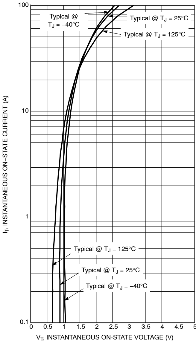
Figure 3. On-State Characteristics
