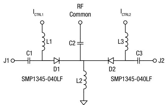
Typical SPDT Switch
