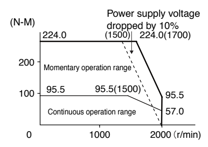
R88M-K15K015C (15 kW)
