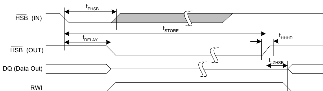
Figure 12. Hardware STORE Cycle [42]
