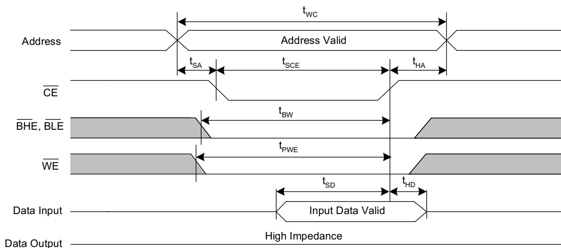
Figure 7. SRAM Write Cycle #2 ( \overline{\text{CE}} Controlled) [26, 27, 28, 29]
