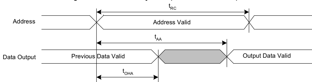
Figure 4. SRAM Read Cycle #1 (Address Controlled) [14, 15, 19]
