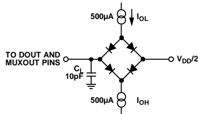
Figure 3. Load Circuit for DOUT/MUXOUT Timing, C_L = 10\text{pF}
