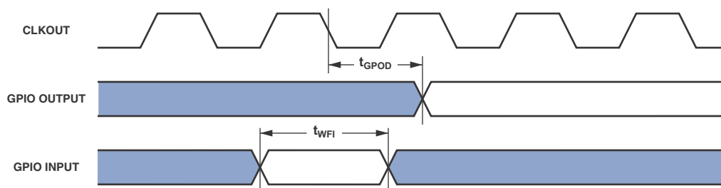
Figure 25. General-Purpose Port Timing
