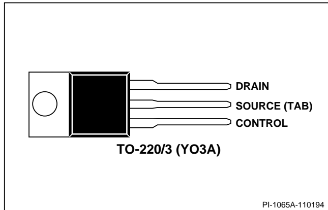
Figure 3. Pin Configuration.
