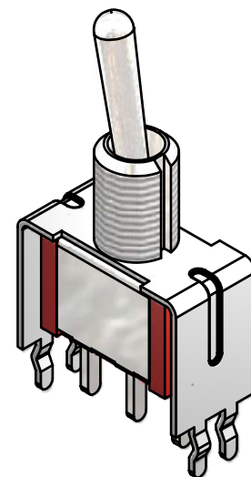
ISOMETRIC
