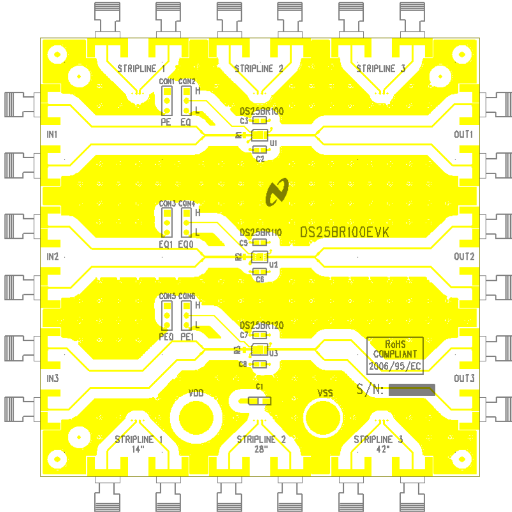
Figure 1. Driver Board
