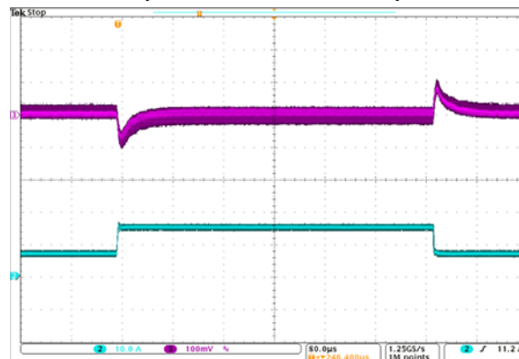
24Vin to 1.8Vout, Cout = 8X 100μF Ceramic
