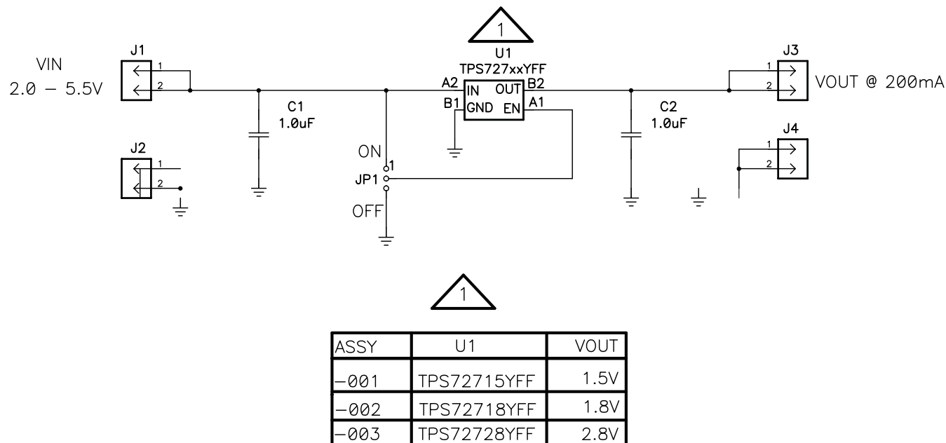
Figure 5. TPS727xxYFFEVM-407 Schematic
