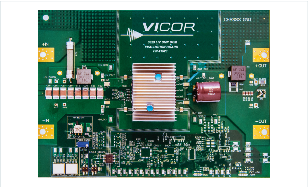
Figure 1. 3623 DCM evaluation board photo, top side
