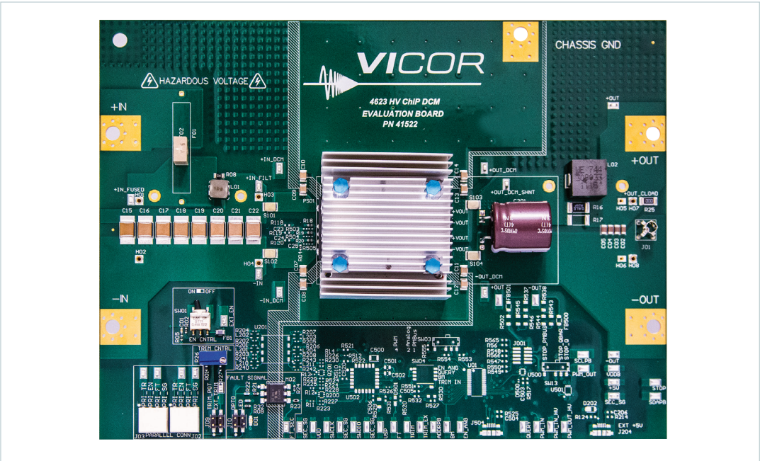
Figure 2. 4623 DCM evaluation board photo, top side
