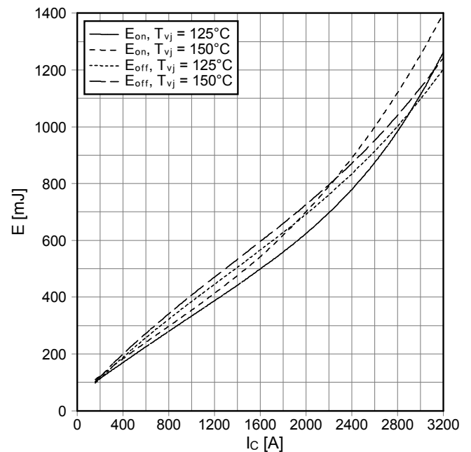
Schaltverluste IGBT-Wechselr. (typisch) switching losses IGBT-inverter (typical) E_{on} = f(I_c), E_{off} = f(I_c) V_{GE} = \pm 15\text{ V}, R_{Gon} = 0.8\ \Omega, R_{Goff} = 0.6\ \Omega, V_{CE} = 900\text{ V}
