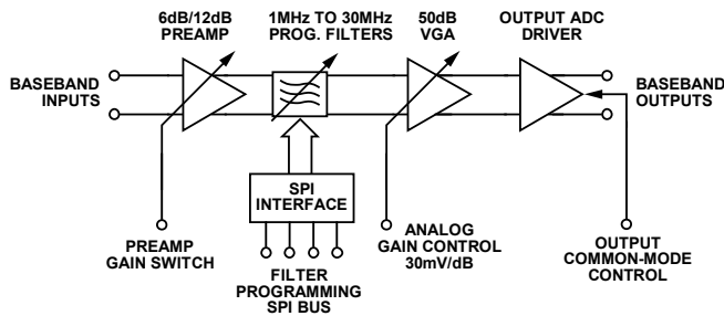
Figure 42. Signal Path Block Diagram for a Single Channel of the ADRF6510
