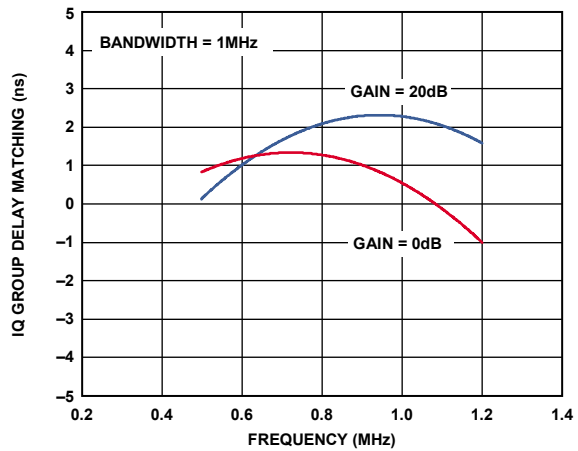
Figure 16. IQ Group Delay Mismatch vs. Frequency (Bandwidth Setting = 1 MHz)
