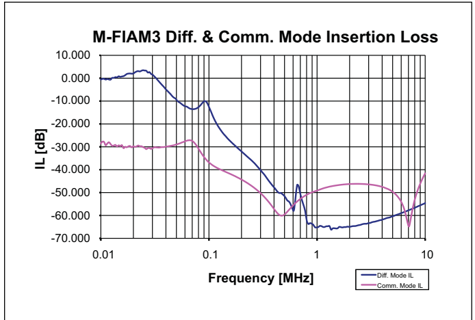
Figure 4–Insertion Loss Curve
