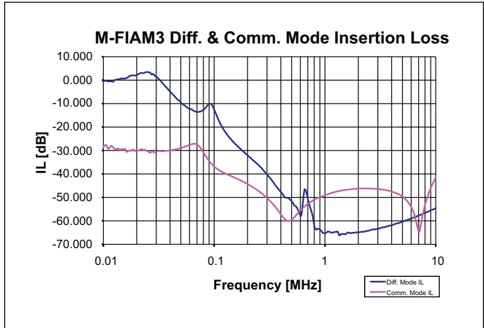
Figure 4–Insertion Loss Curve
