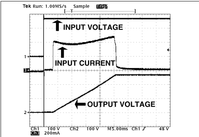
Figure 3–Inrush Limiting; Inrush current with 22 \mu F external capacitance, (C1 in Figure 5)
